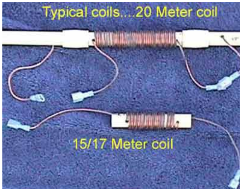
Photo 1: Coil Details
